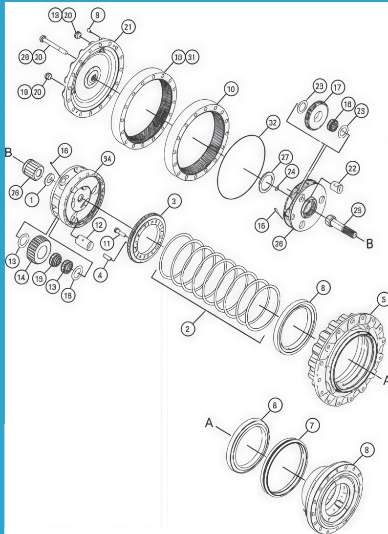
Travel planetary carrier
